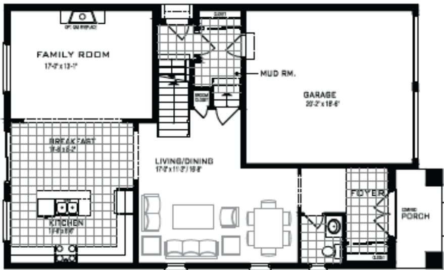
FIRST FLOOR PLAN EL-A
