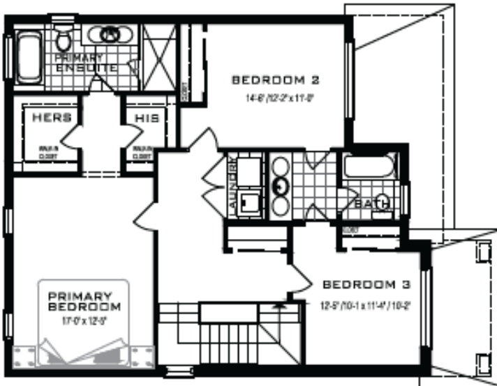
SECOND FLOOR PLAN ELEVATION A
