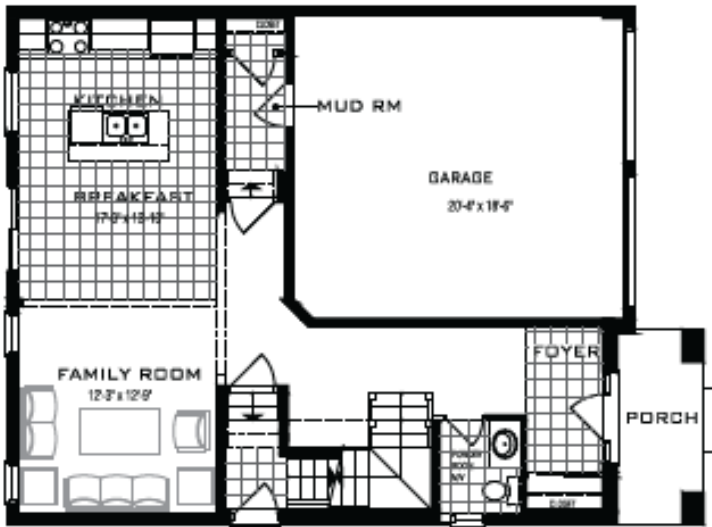
FIRST FLOOR PLAN ELEVATION A
