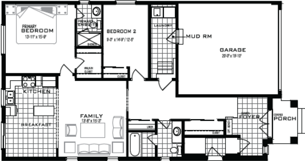
FIRST FLOOR PLAN ELEVATION A
