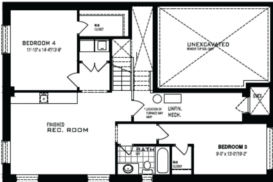
FINISHED BASEMENT PLAN ELEVATION A & B
